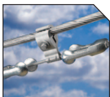
Stockbridge Vibration Dampers
